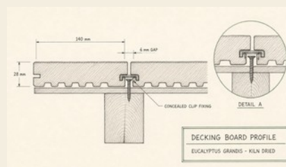
DECKING BOARD PROFILE
