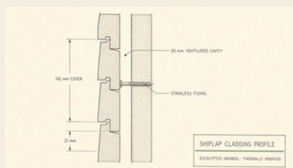
SHIPLAP CLADDING PROFILE
